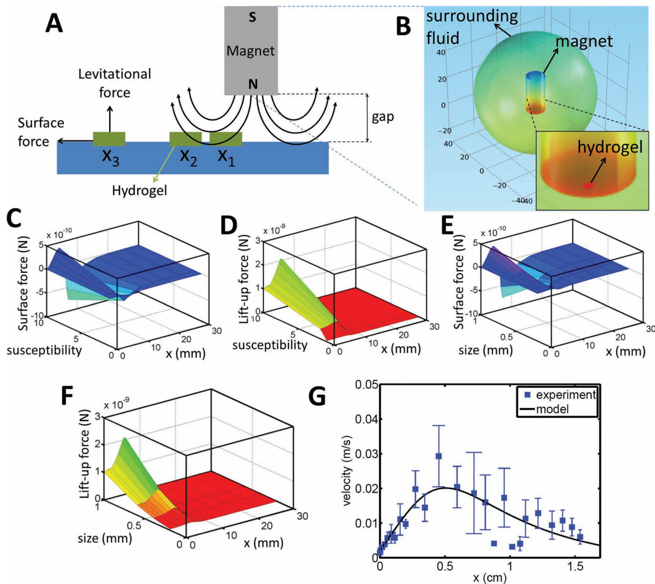
Figure 2. (A) Schematic for the motion of a hydrogel ( 1 \text{ mm} \times 1 \text{ mm} \times 200 \mu\text{m} ) under a magnetic field. (B) Contour plot of magnetic potential. (C) Surface and (D) Levitational magnetic forces as a function of hydrogel susceptibility and horizontal “x” location. (E) Surface and (F) Levitational magnetic forces as a function of characteristic length of a hydrogel and horizontal “x” location. (G) Validation of hydrogel motion as a function of time (squares represent experimental data ( n = 10 ) and solid line represents the model fit).
